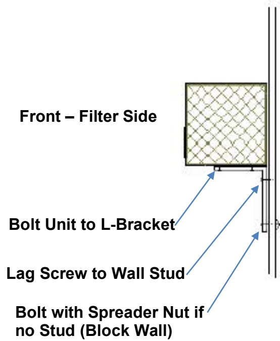
L-Bracket Installed
